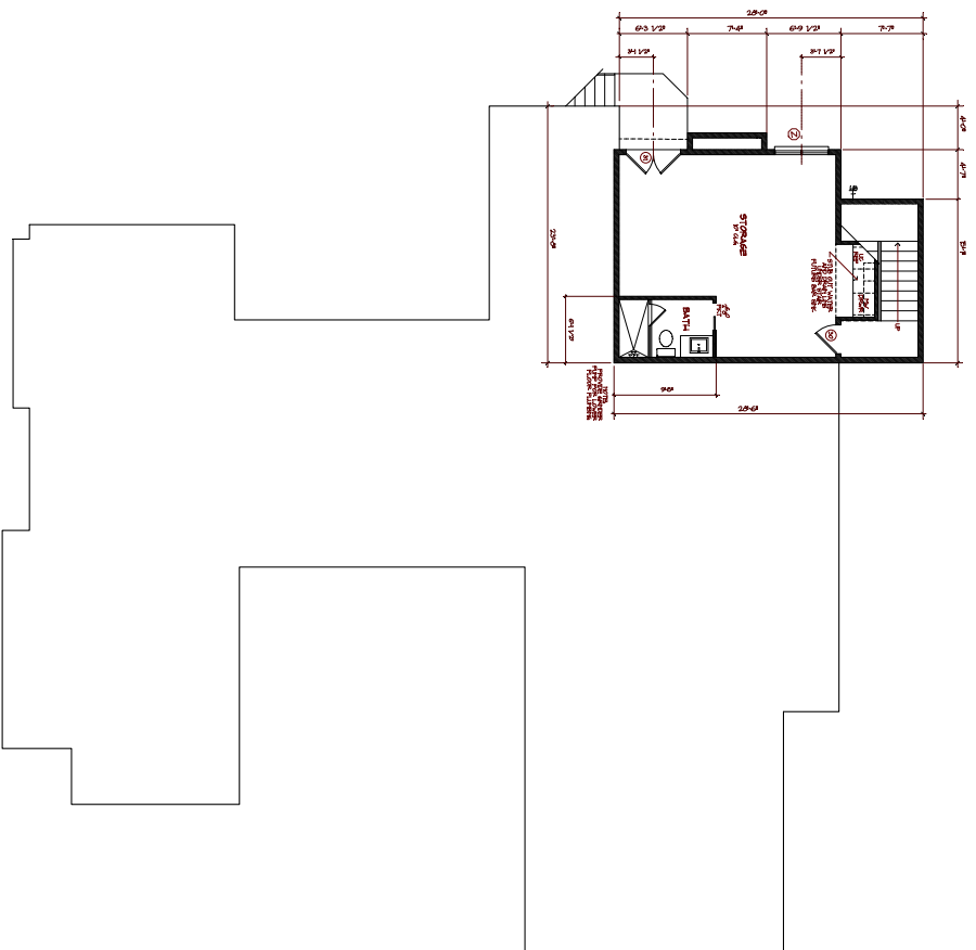
LOWER FLOOR PLAN 537 SQ FT
